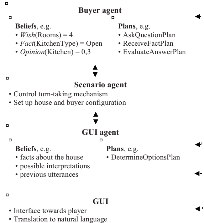
Figure 2. Agent architecture
